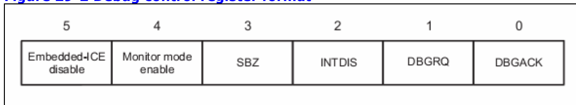
Figure 29-2 Debug control register format
