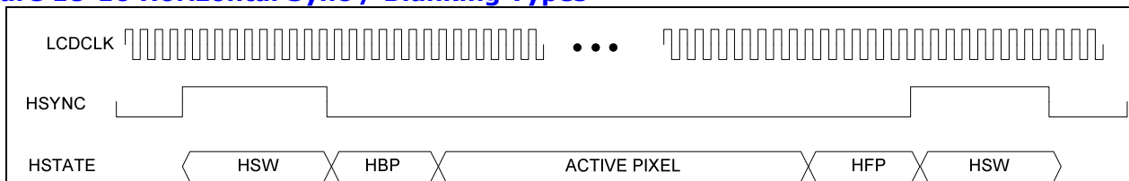
Figure 18-10 Horizontal Sync / Blanking Types
