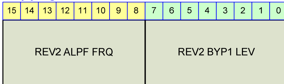
Figure 23-85 REV2(6) Register
