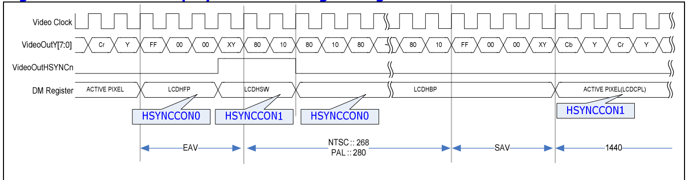
Figure 17-14 BT656 Display module Timing setting
