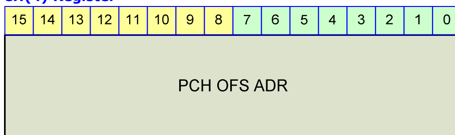
Figure 23-62 PCH(4) Register
