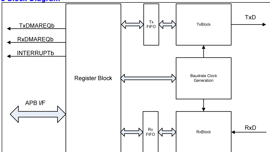
Figure 21-1 Block Diagram
