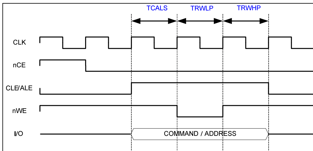
Figure 9-3 ALE,CLE Timing
