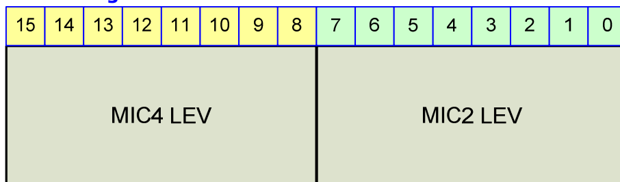
Figure 23-45 MIC LEV Register
