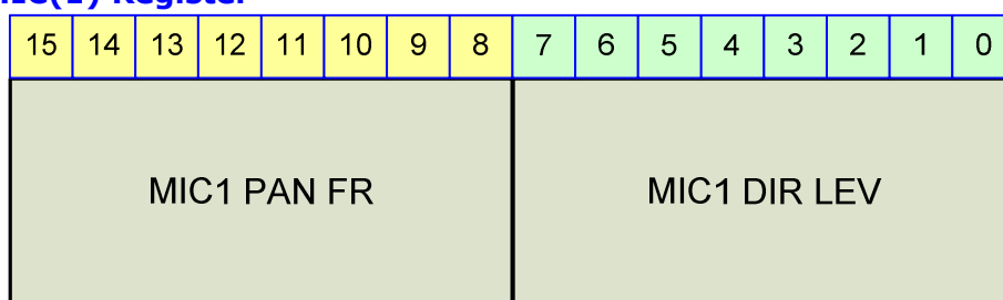
Figure 23-48 MIC(1) Register
