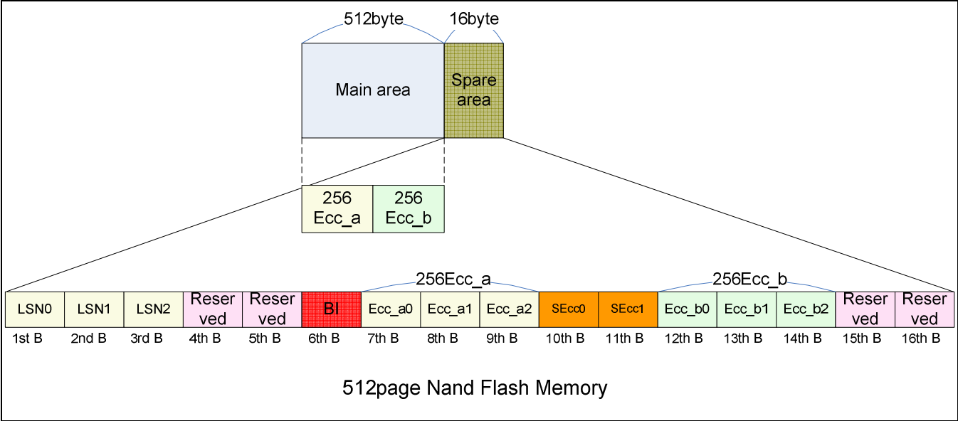
Figure 9-19 Spare area
