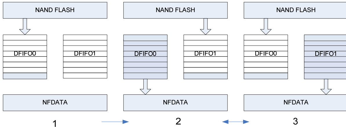
Figure 9-22 Data FIFO(read)
