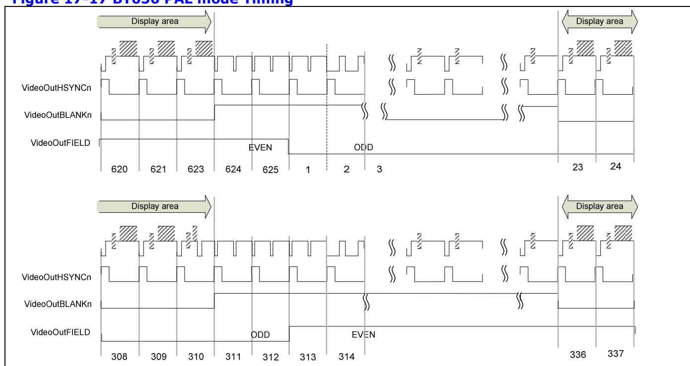
Figure 17-17 BT656 PAL mode Timing
