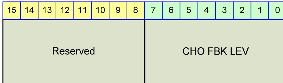
Figure 23-58 CHO (7) Register
