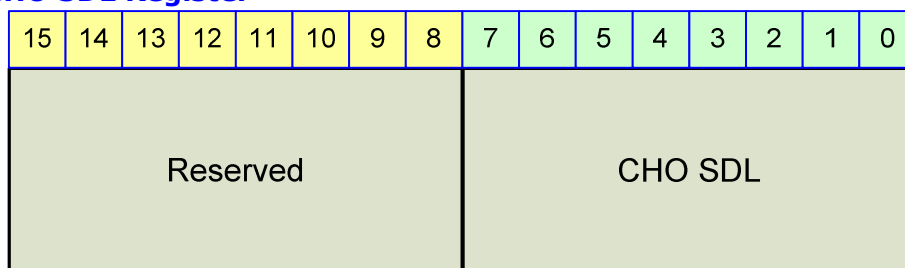
Figure 23-32 CHO SDL Register
