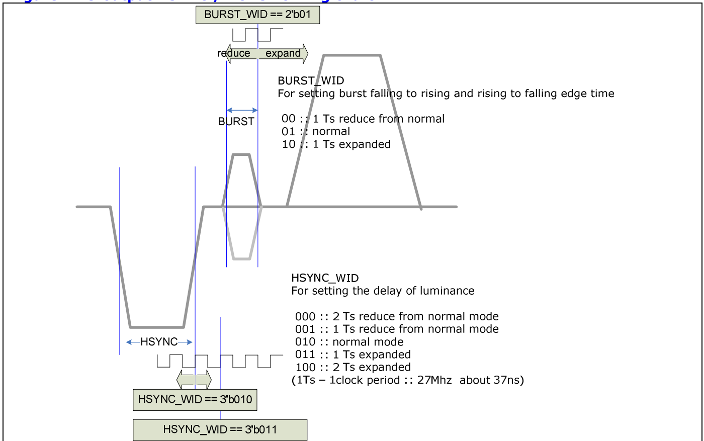
Figure 17-9 output HSYNC / BURST timing chart
