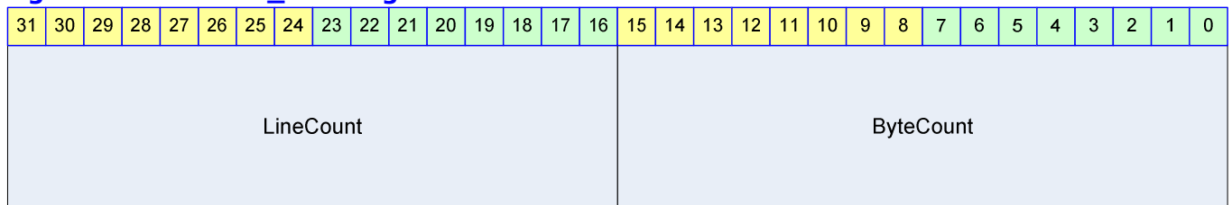
Figure 12-8 DMA2D_CNT Register
