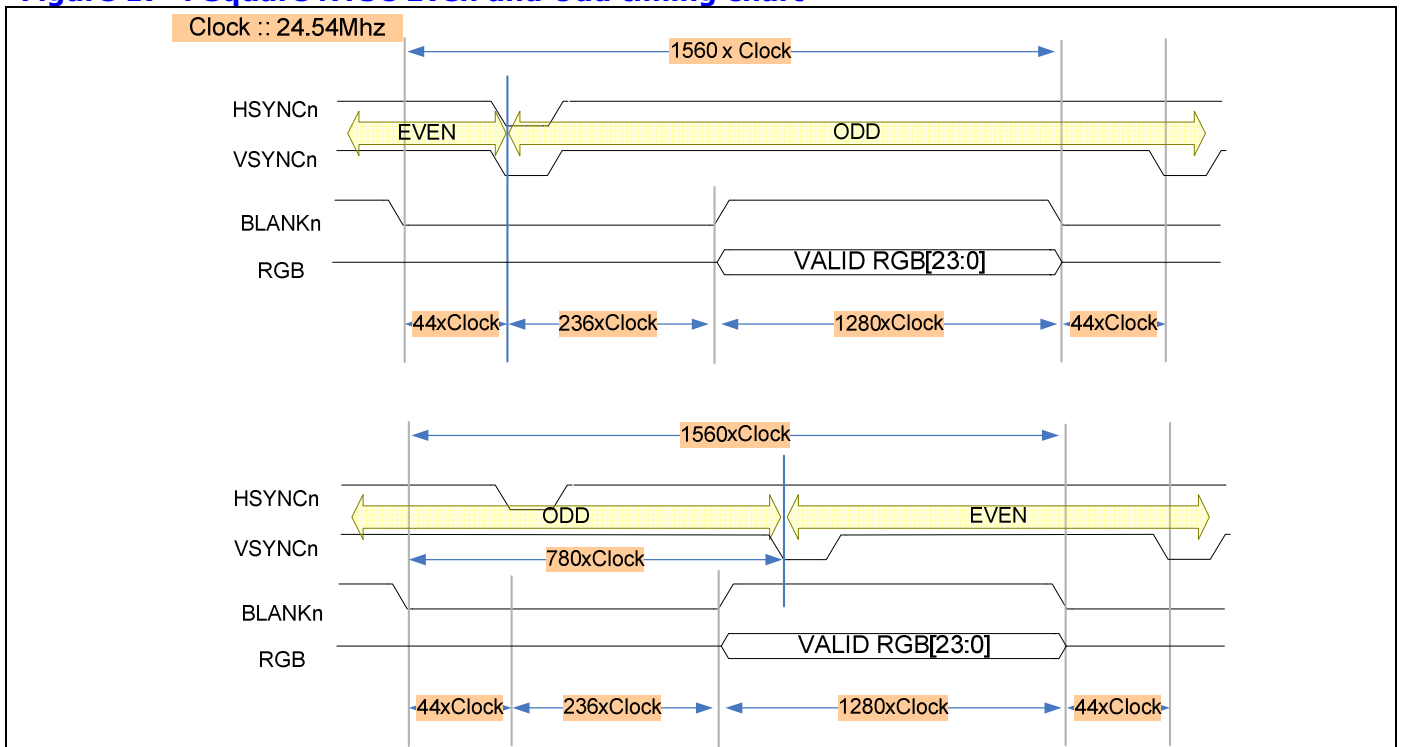
Figure 17-4 Square NTSC Even and Odd timing chart
