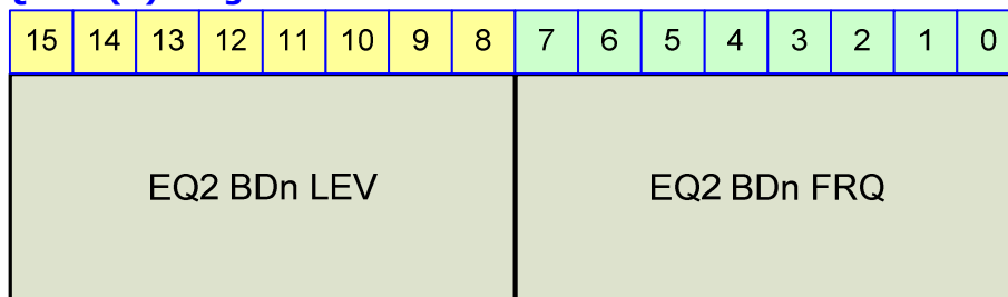
Figure 23-47 EQ2 BD(n) Register
