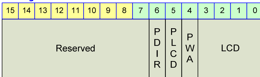
Figure 23-18 INIT Register
