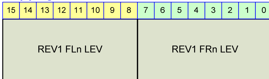
Figure 23-76 REV1(8) Register
