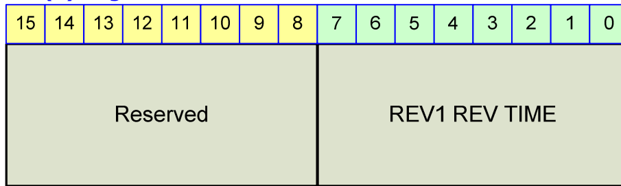
Figure 23-75 REV1(7) Register
