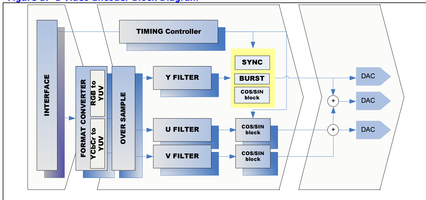
Figure 17-1 Video Encoder Block Diagram
