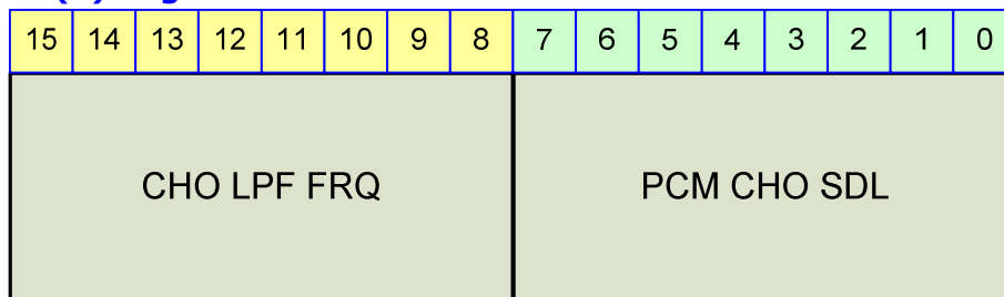
Figure 23-52 CHO(1) Register
