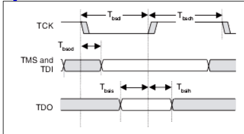
Figure 27-1 JTAG signal standard wave
