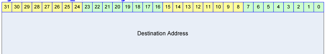
Figure 12-6 DMA2D_DSTADDR Register
