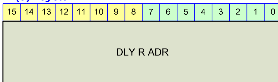
Figure 23-98 ADR(5) Register
