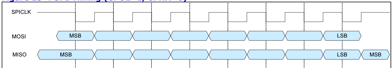
Figure 25-4 SPI Timing (CPOL=1, CPHA=0)
