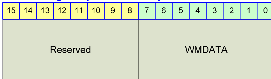
Figure 23-16 WMDT Register (address : 044H)
