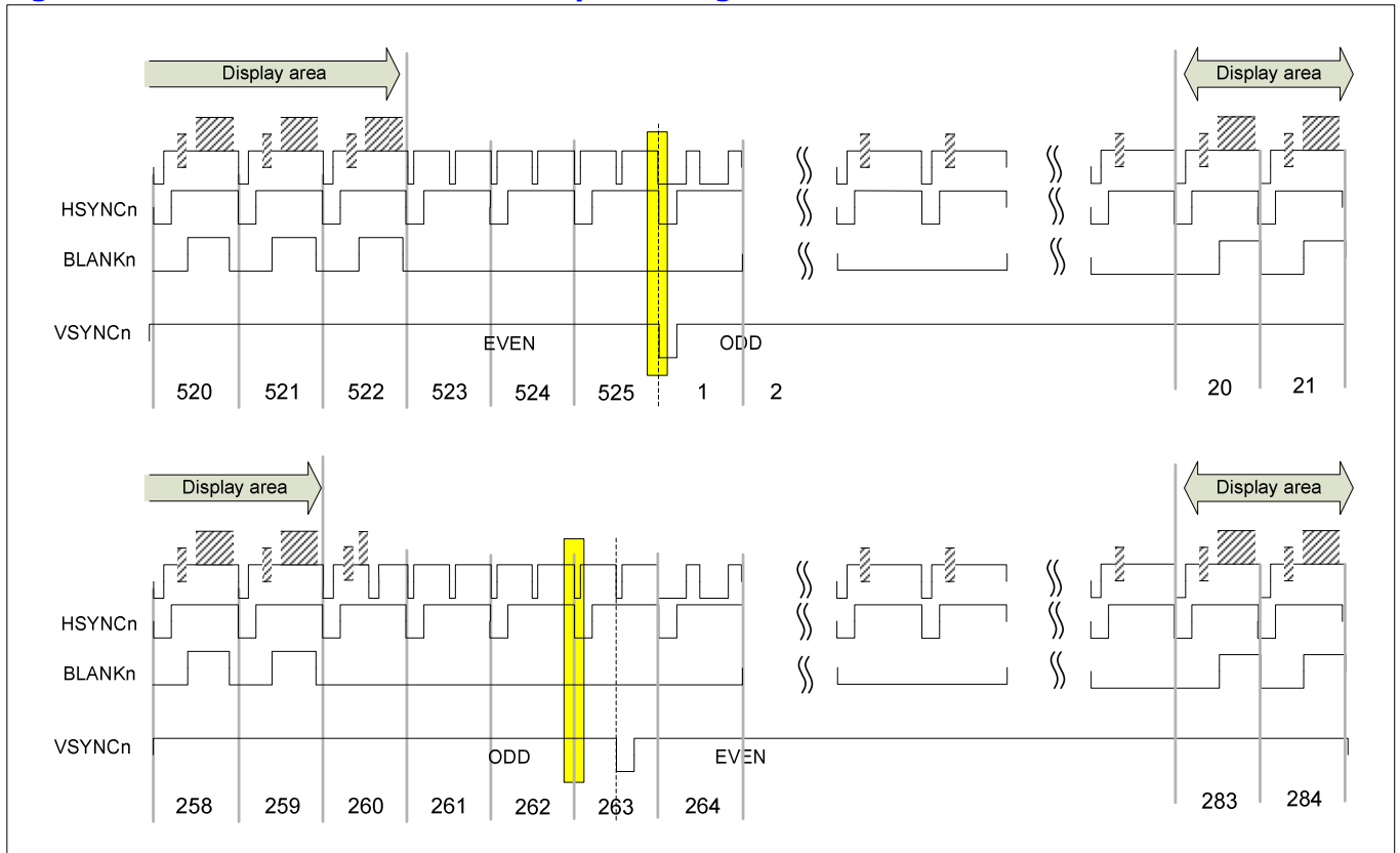
Figure 17-2 Interlaced NTSC Video input timing chart
