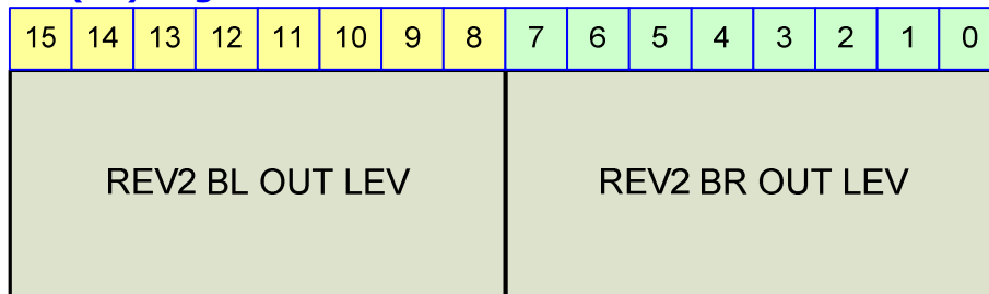
Figure 23-90 REV2(11) Register
