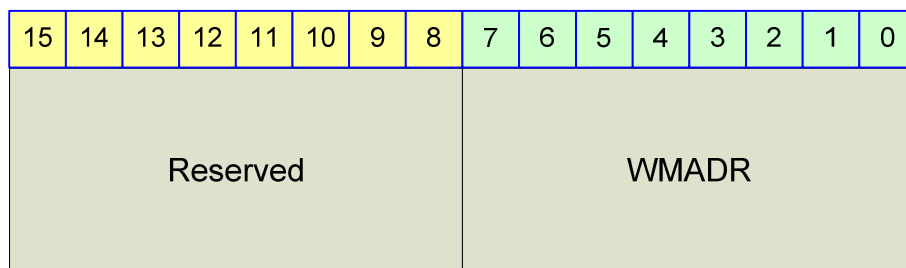
Figure 23-14 WMAL Register(address : 040H)
