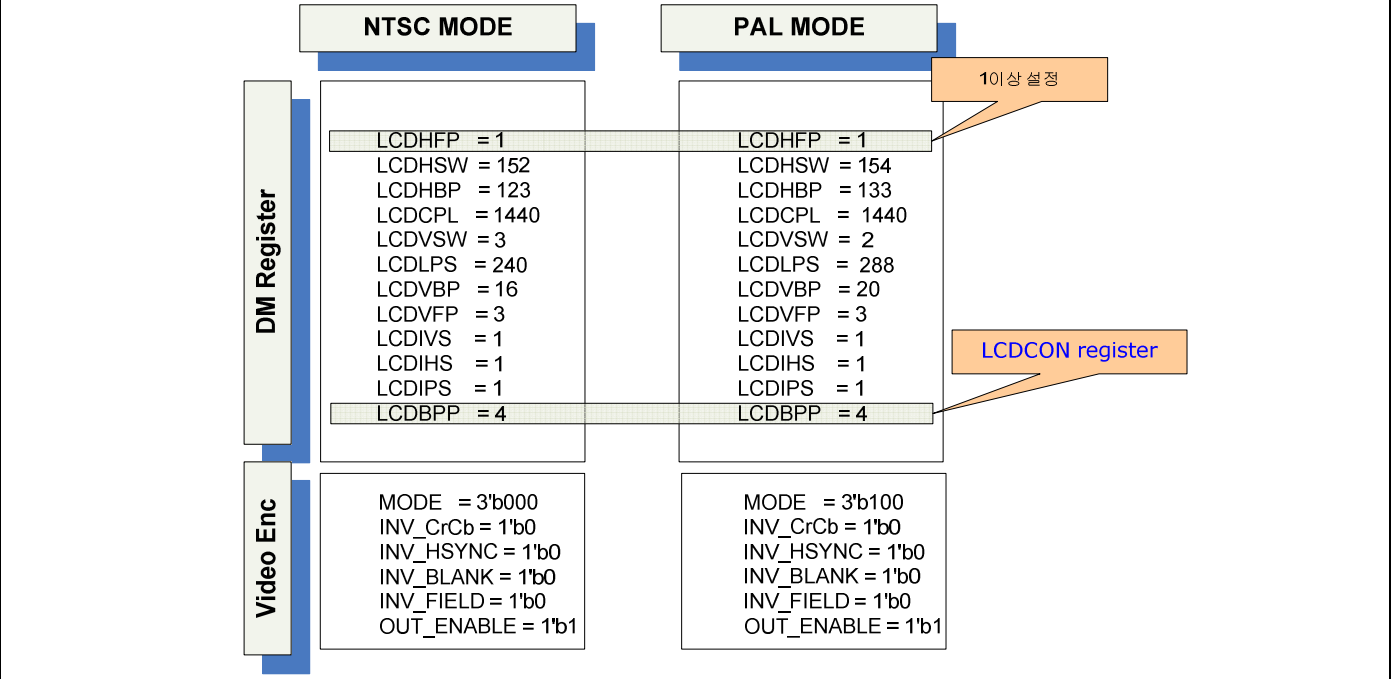
Figure 17-18 BT656 mode register setting example (decimal value)
