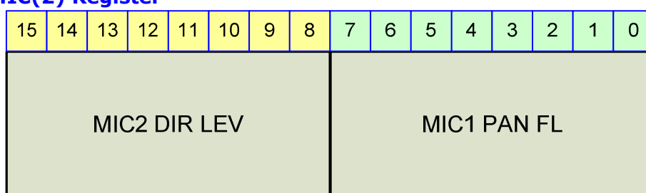
Figure 23-49 MIC(2) Register
