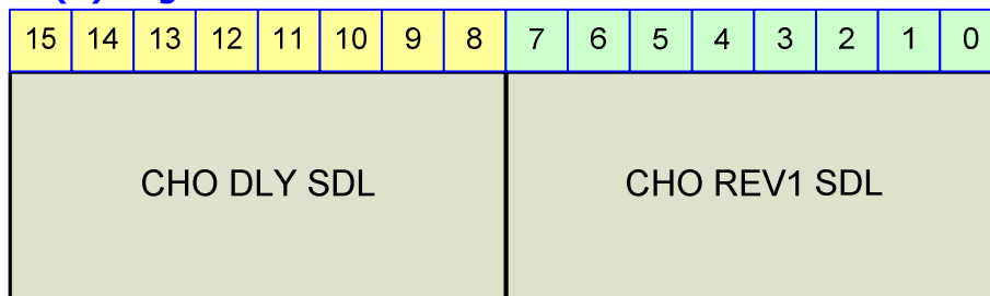
Figure 23-57 CHO(6) Register
