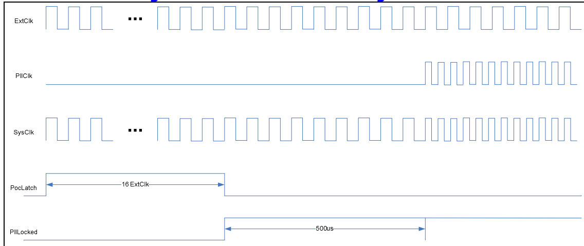
Figure 6-4 Power On Configuration & PLL Lock Time Diagram
