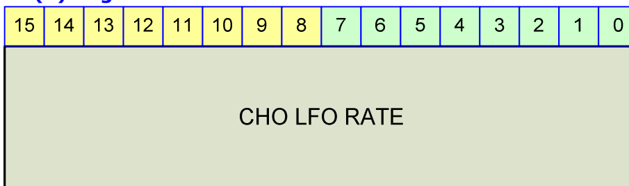
Figure 23-53 CHO(2) Register
