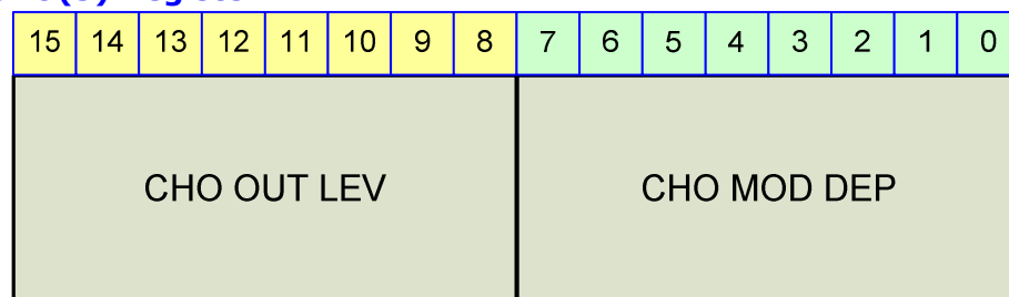
Figure 23-56 CHO(5) Register
