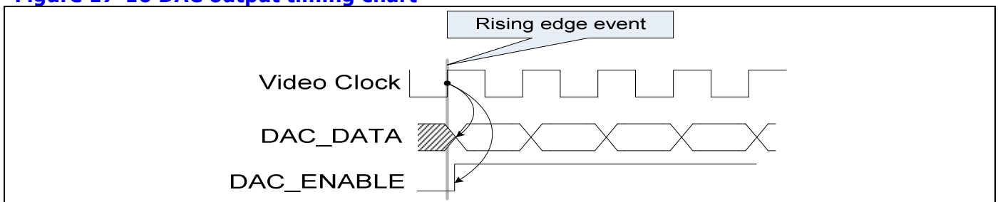
Figure 17-10 DAC output timing chart
