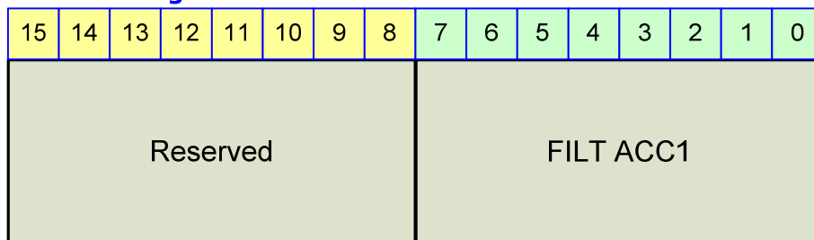
Figure 23-26 FILT ACC1 Register
