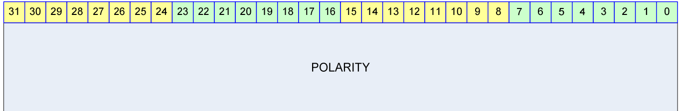
Figure 10-8 POLARITY Register
