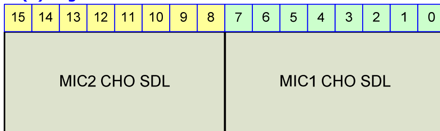
Figure 23-51 MIC(4) Register
