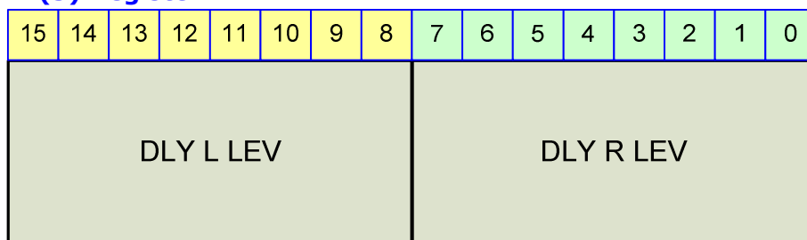
Figure 23-67 DLY(3) Register
