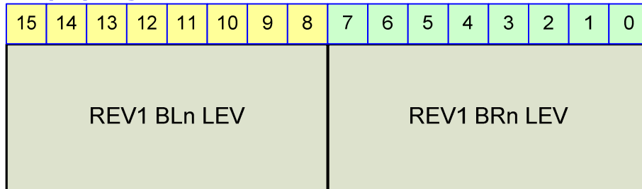
Figure 23-78 REV1(10) Register
