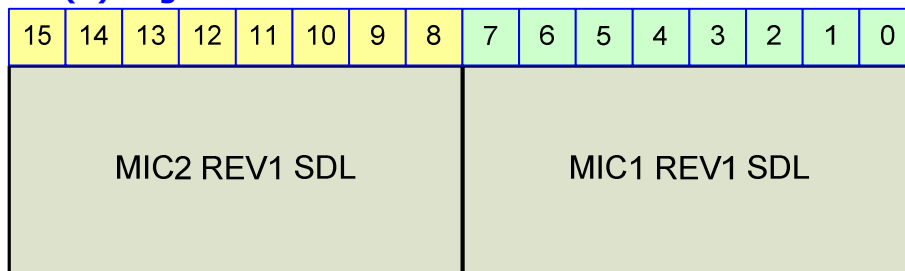
Figure 23-69 REV1(1) Register
