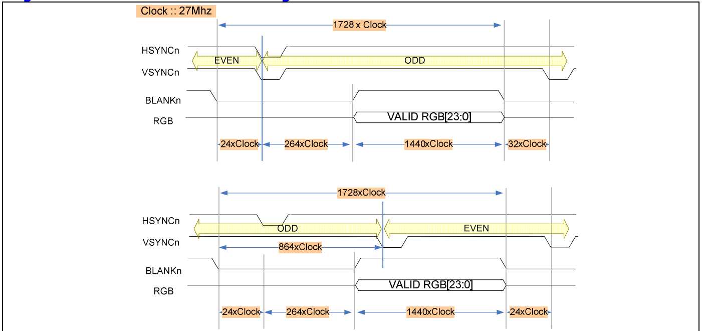
Figure 17-7 PAL Even and Odd timing chart
