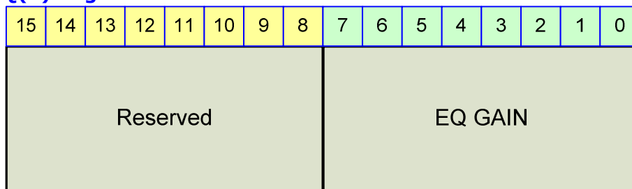
Figure 23-91 EQ(1) Register
