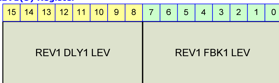
Figure 23-73 REV1(5) Register
