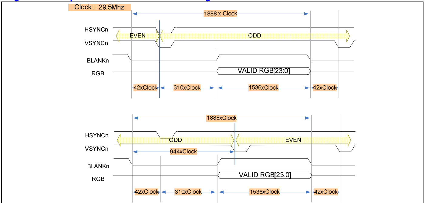
Figure 17-8 Square PAL Even and Odd timing chart
