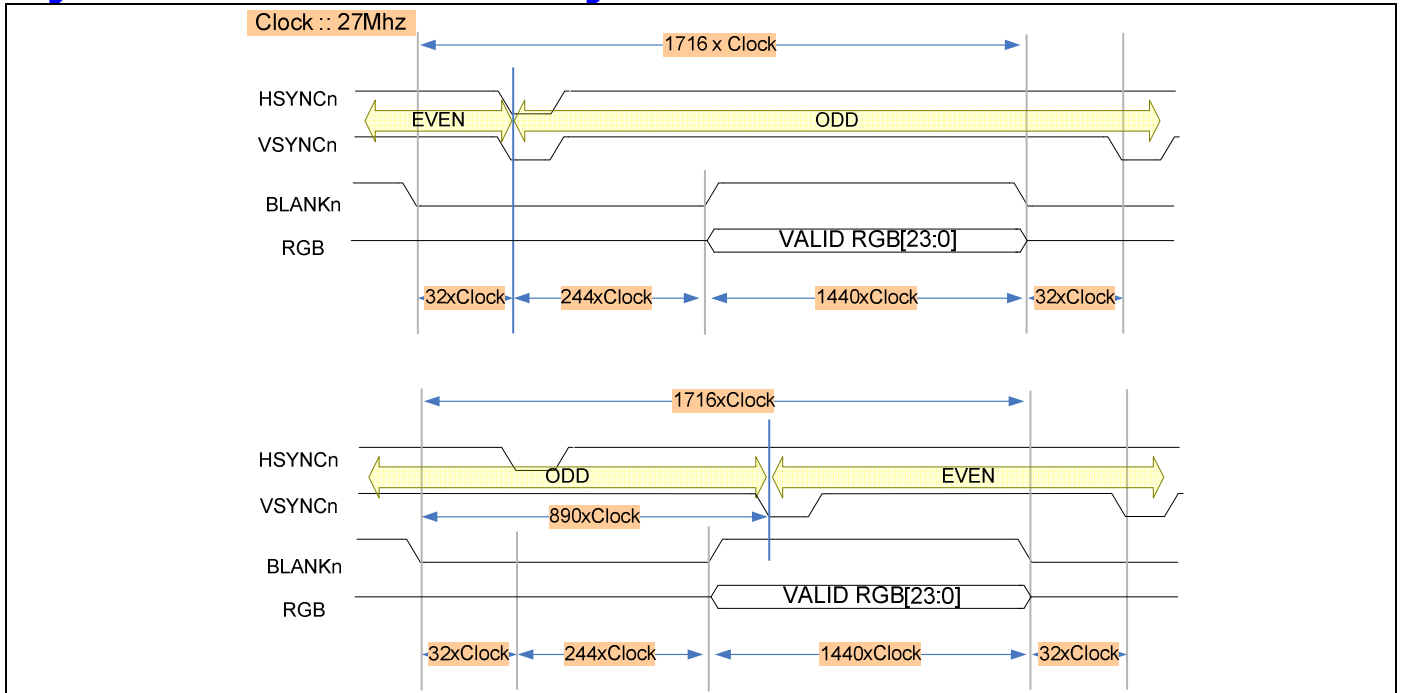
Figure 17-3 NTSC Even and Odd timing chart
