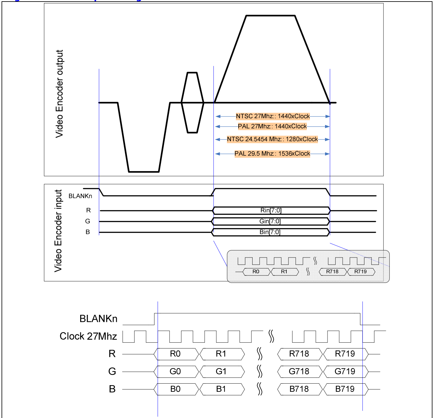
Figure 17-5 RGB input timing
