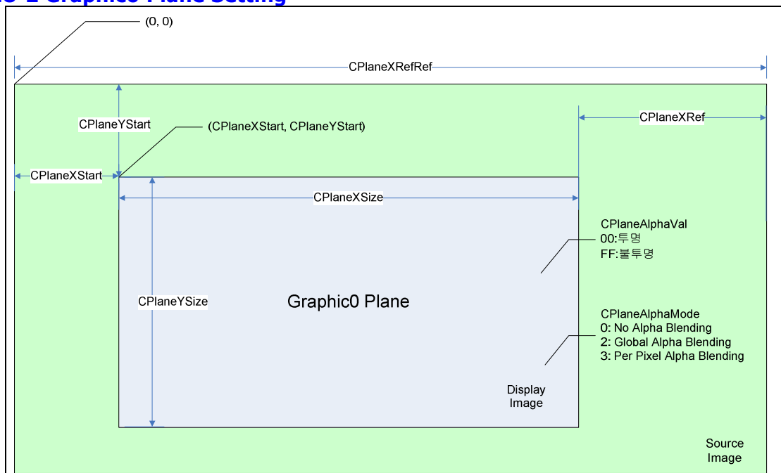
Figure 18-2 Graphic0 Plane Setting
