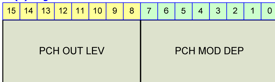
Figure 23-63 PCH(5) Register
