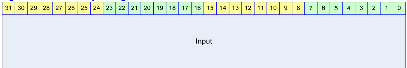
Figure 24-4 GPIO Input Register
