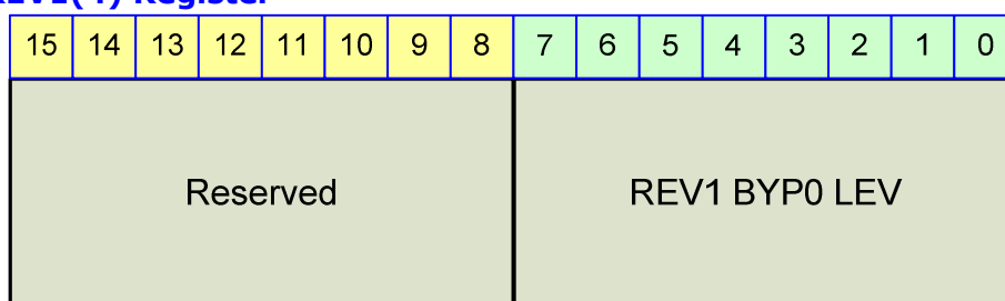
Figure 23-72 REV1(4) Register
