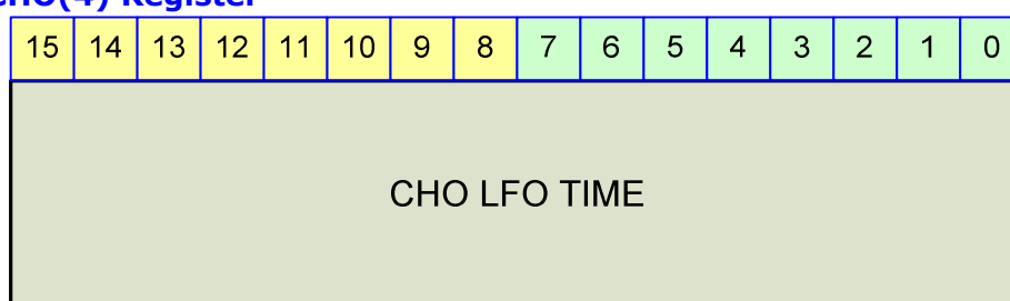
Figure 23-55 CHO(4) Register
