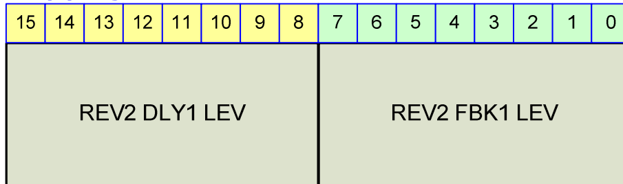
Figure 23-84 REV2(5) Register
