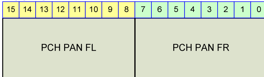
Figure 23-64 PCH(6) Register
