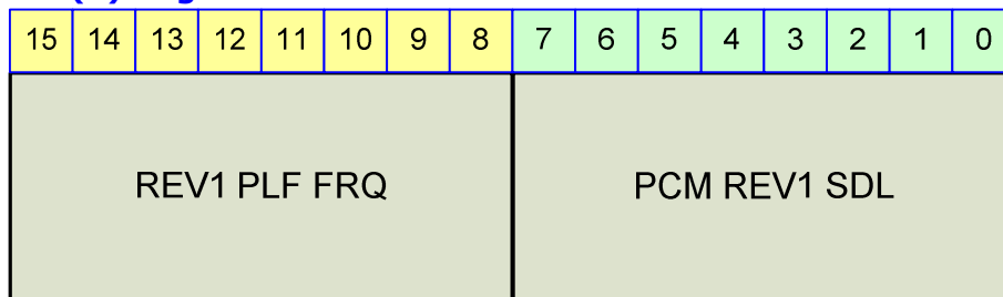
Figure 23-70 REV1(2) Register
