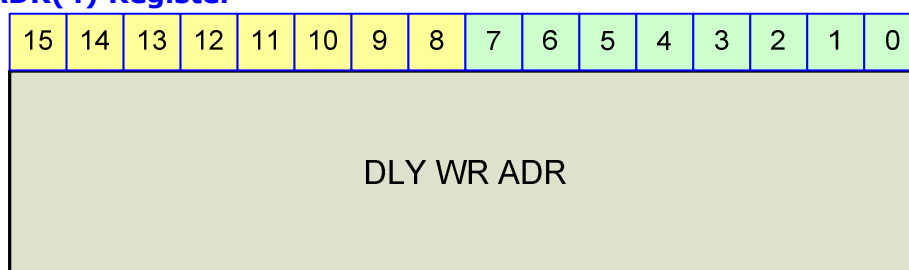
Figure 23-97 ADR(4) Register
