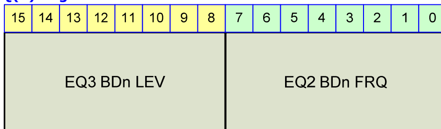
Figure 23-92 EQ(2) Register
