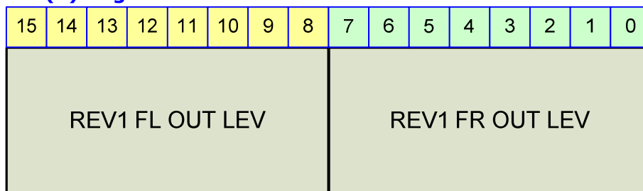
Figure 23-77 REV1(9) Register
