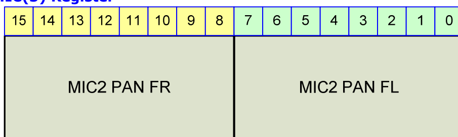
Figure 23-50 MIC(3) Register
