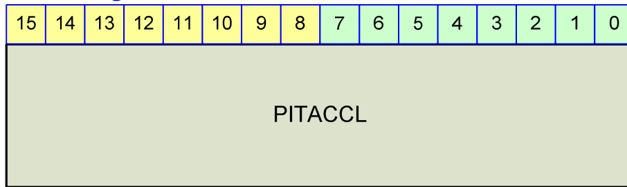
Figure 23-24 PITACCL Register
