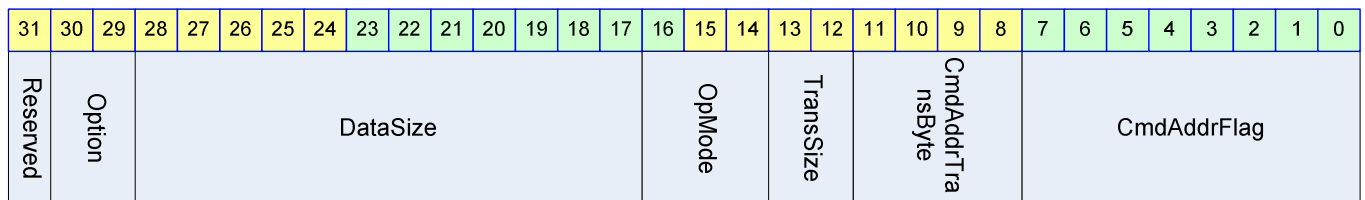
Figure 9-6 1 st Operation Register bit
