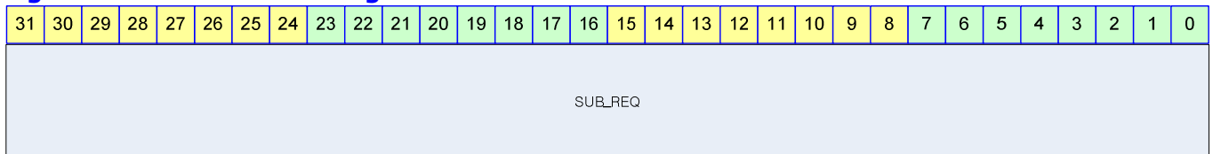
Figure 17-23 Subcarrier Register Bits
