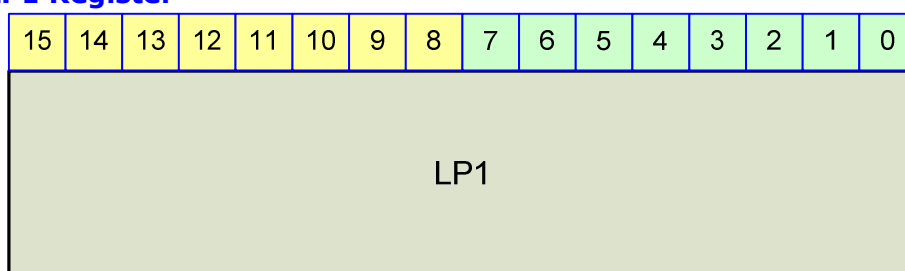
Figure 23-21 LP1 Register
