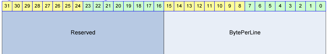
Figure 12-7 DMA2D_SIZE Register
