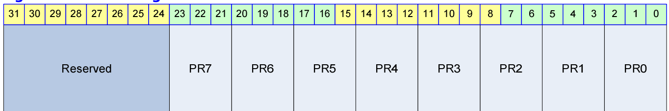
Figure 10-9 PSLV Register
