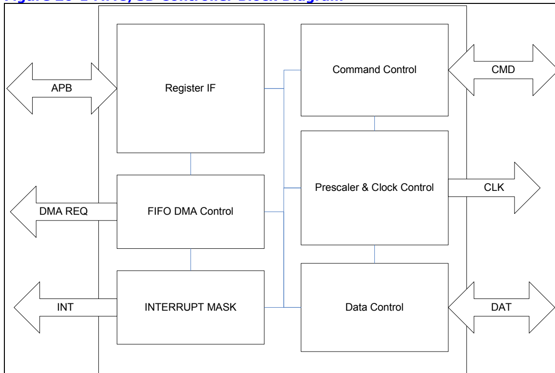
Figure 26-1 MMC/SD Controller Block Diagram
