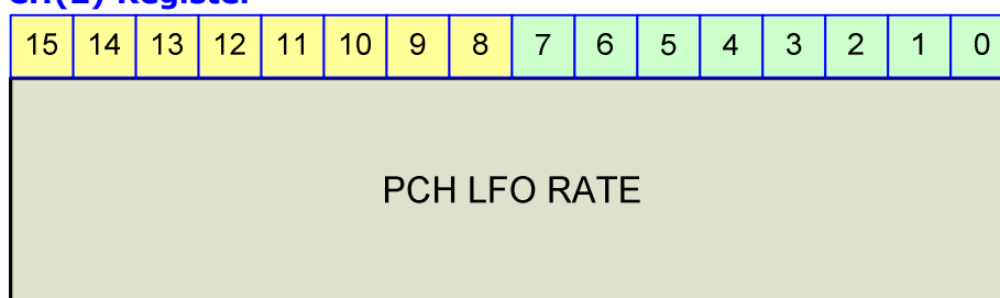
Figure 23-60 PCH(2) Register
