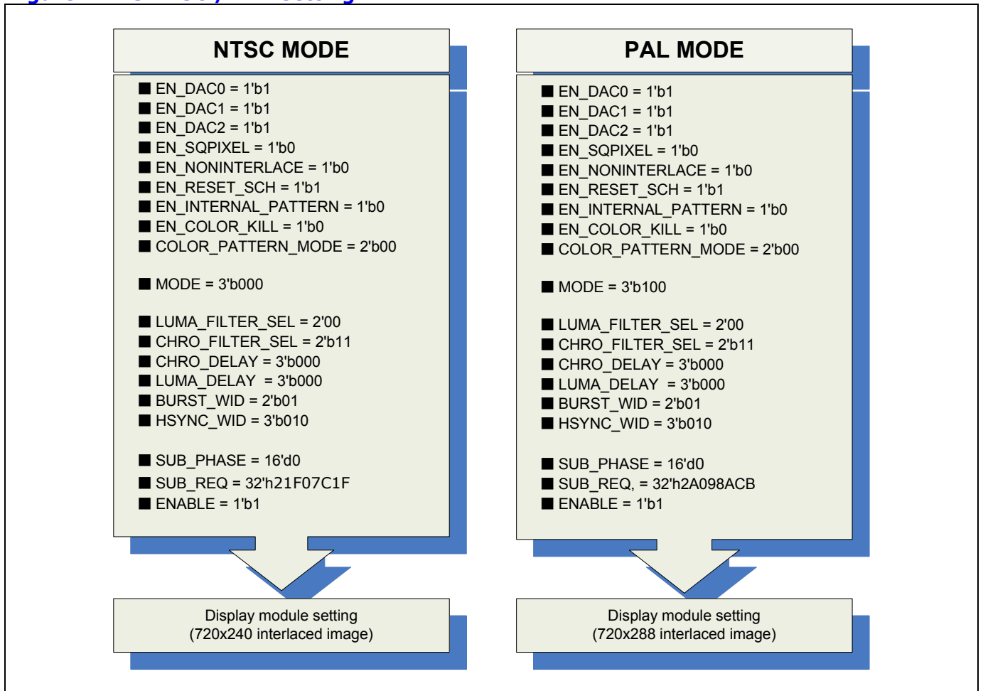
Figure 17-13 NTSC / PAL setting
