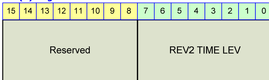
Figure 23-86 REV2(7) Register
