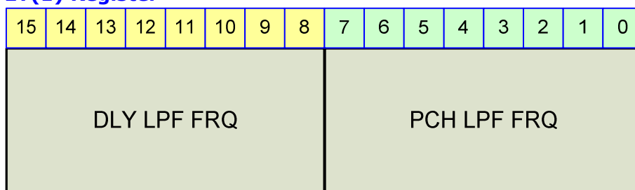
Figure 23-65 DLY(1) Register
