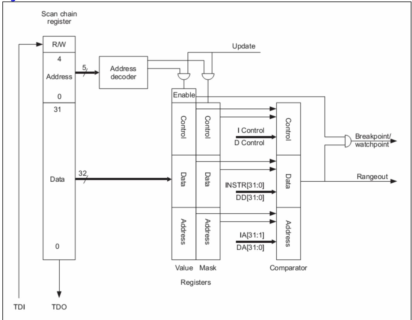
Figure 29-1 EmbeddedICE-RT macrocell overview
