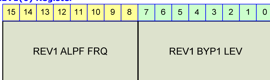
Figure 23-74 REV1(6) Register
