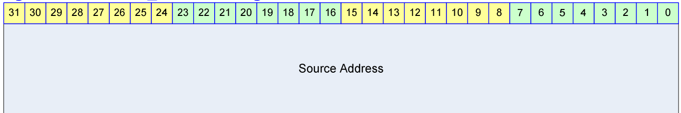
Figure 12-5 DMA2D_SRCADDR Register
