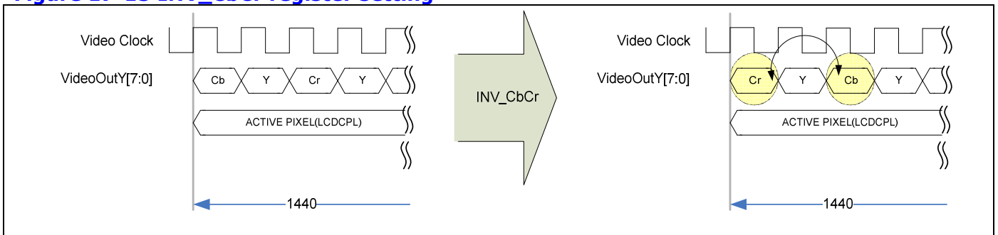
Figure 17-15 INV_CbCr register setting
