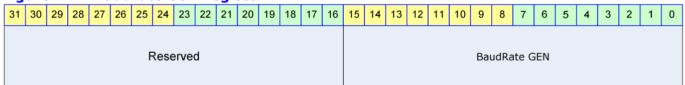
Figure 21-4 Baudrate Gen Register
